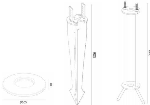
Add-on base
